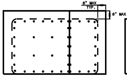
IF OVERLAYING SIGN OVERLAPS SIGN ON TOP AND SIDES DETAIL NO.2
