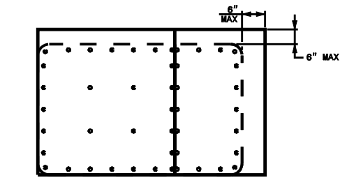
IF OVERLAYING SIGN OVERLAPS SIGN ON TOP AND ONE SIDE DETAIL NO.8
