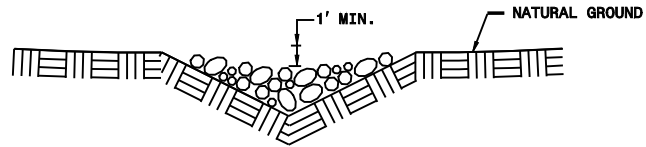
CROSS SECTION VEE DITCH
