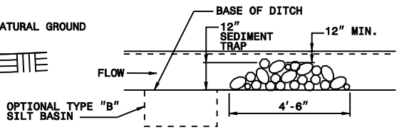
ELEVATION VIEW
