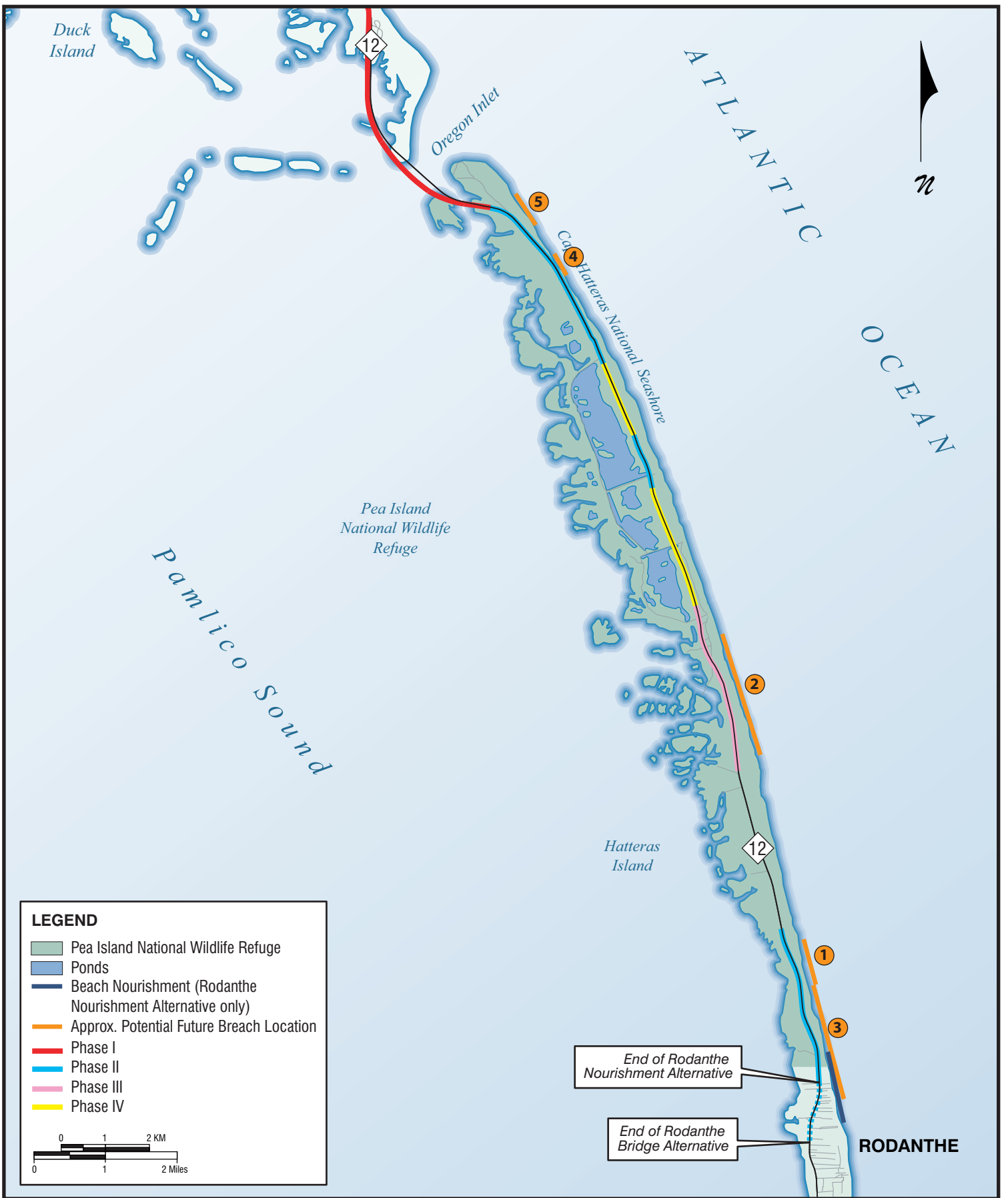
PARALLEL BRIDGE CORRIDOR WITH PHASED APPROACH
